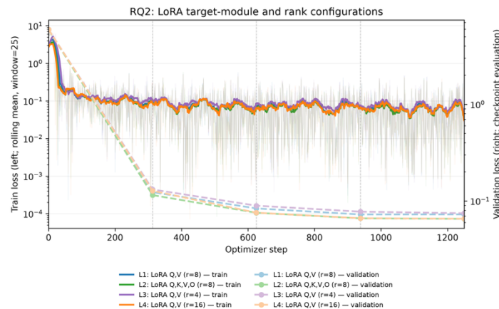
Figure 4. Training and Validation Loss across LoRA Target Module and Rank Configurations
